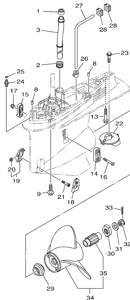
NORMAL PROPELLER
