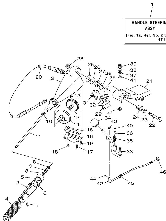
THROTTLE FRICTION
